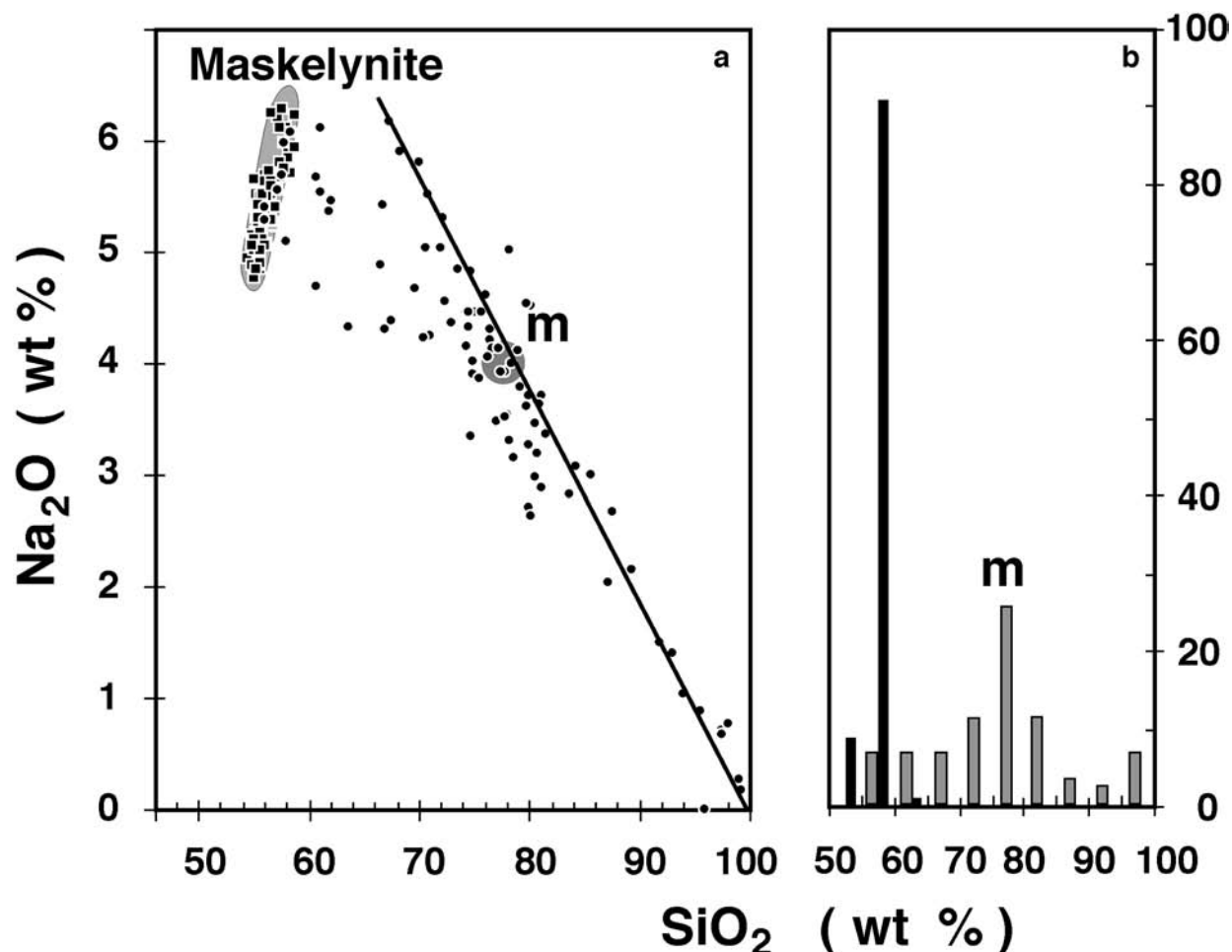
FIG. 8. Composition of silica-maskelynite patches associated with maskelynite. (a) The straight line is a visual fit to the SiO 2 > 80% data points. For SiO 2 < 80%, some of the data points correspond to a mixture of maskelynite and some component ( m ) at 80% silica; they are likely to be an artifact related to the size of the analytical spot (10 \mu m). The trend to a sodium-rich component (the straight line) is expected for a melt derived from silica and maskelynite. (b) The histogram of SiO 2 concentrations reveals, beside maskelynite, a subsidiary maximum corresponding to the most likely melt composition ( m ) in the plagioclase–silica system.
