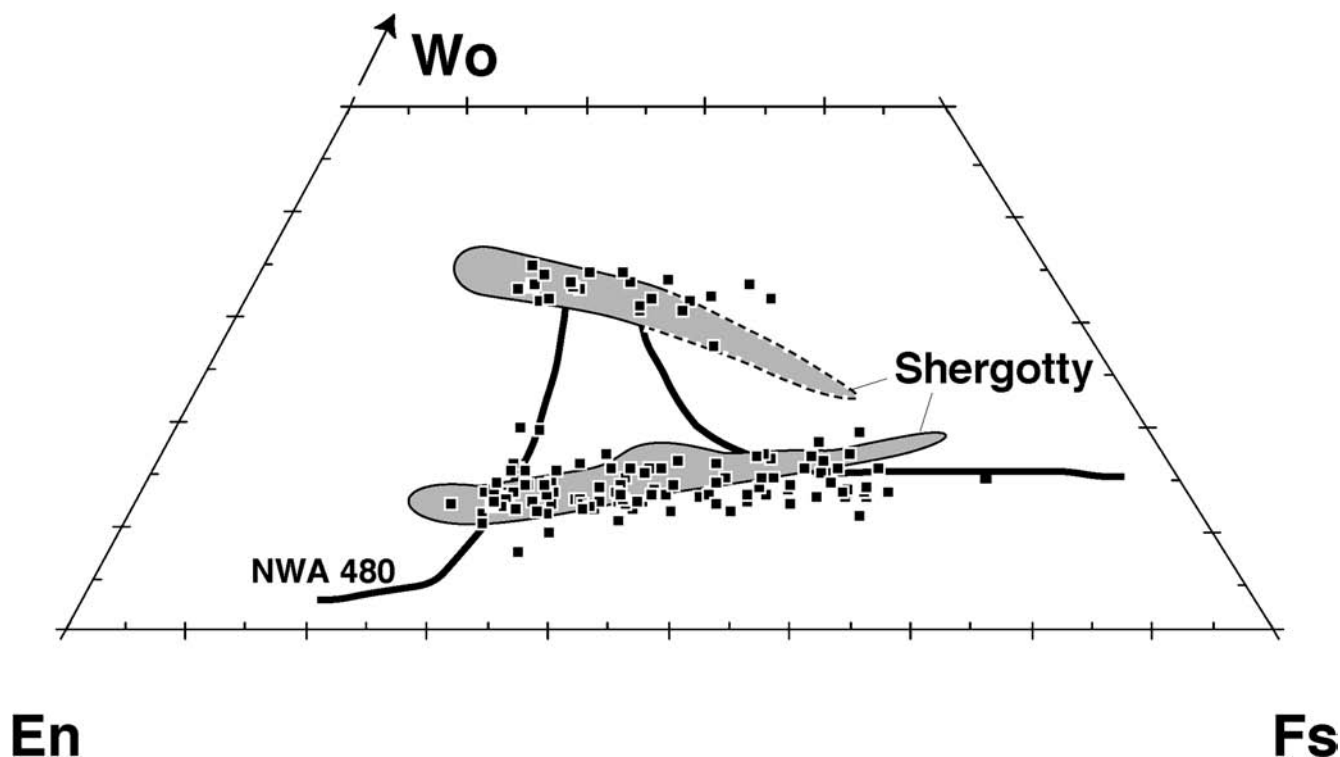
FIG. 6. Quadrilateral pyroxene compositions of NWA 856 compared to Shergotty (shaded area). Data sources are Stöffler et al. (1986), Stolper and McSween (1979), and Smith and Hervig (1979). The line corresponds to the zoning trend observed in shergottite NWA 480 (Barrat et al. , 2002).
