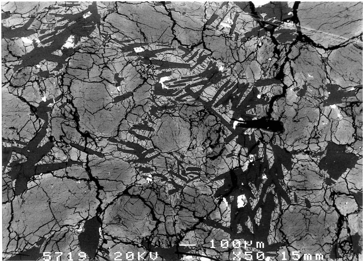
FIG. 3. Backscattered electron image (middle left of the section in Fig. 2) showing the characteristic features. Large grey crystals are zoned pyroxenes, the dark phase is maskelynite. Fe-Ti oxides, minor pyrrhotite and chromite (all white) are included in maskelynite or interstitial between maskelynite and pyroxene. Silica and silica-maskelynite glass (black) inside the maskelynite stacks. Notice the fracturation of pyroxene. Width of view is 1.5 mm.
