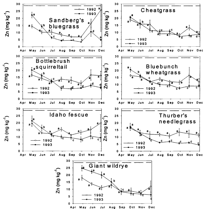
Fig. 7. Mean zinc content ( \pm SE bars) of 7 grasses sampled over 8 months at 6 sites in the sagebrush steppe near Burns, Ore. in 1992 and 1993. The required zinc content of forages for a 454 kg cow is 28.8 \text{ mg kg}^{-1} (dashed horizontal line). Adjacent monthly means within a year sharing a common letter are not significantly different ( P > 0.05 ). Fisher's protected LSD ( P = 0.05 ) = 7.82 and 3.75 \text{ mg kg}^{-1} , respectively, for 1992 and 1993.
