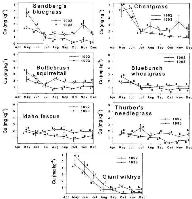
Fig. 6. Mean copper content ( \pm SE bars) of 7 grasses sampled over 8 months at 6 sites in the sagebrush steppe near Burns, Ore. in 1992 and 1993. The required copper content of forages for a 454 kg cow is 9.6 \text{ mg kg}^{-1} . Adjacent monthly means within a year sharing a common letter are not significantly ( P > 0.05 ) different. Fisher's protected LSD ( P = 0.05 ) = 1.19 and 0.73 \text{ mg kg}^{-1} , respectively, for 1992 and 1993.
