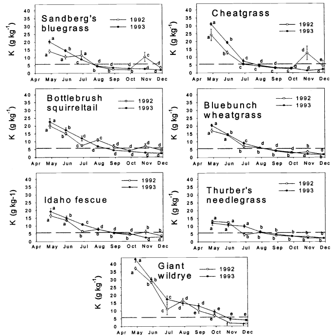
Fig. 5. Mean potassium content ( \pm SE bars) of 7 grasses sampled over 8 months at 6 sites in the sagebrush steppe near Burns, Ore. in 1992 and 1993. The dashed horizontal line denotes required K content of forages for a 454 kg cow. Adjacent monthly means within a year sharing a common letter are not significantly ( P > 0.05 ) different. Fisher's protected LSD ( P = 0.05 ) = 3.77 and 2.56 g \text{kg}^{-1} , respectively, for 1992 and 1993.
