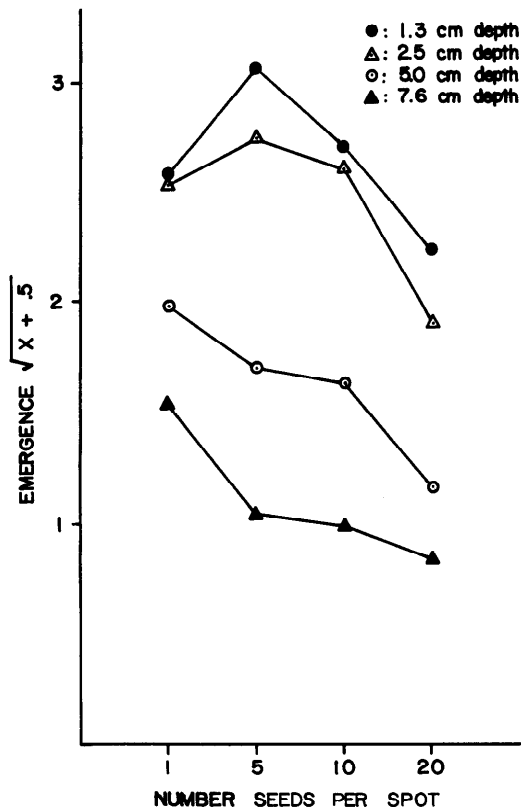
Fig. 1. Bitterbrush emergence as affected by increasing number of seeds/spot at constant depth.
