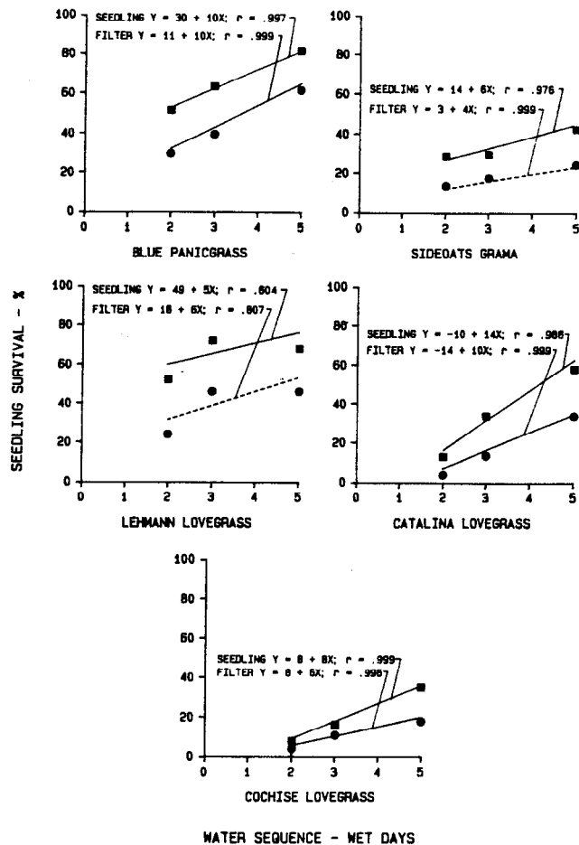
Fig. 4. Seedling survival of 5 grass species in a greenhouse, corrected to filter paper and seedling count (pls) germination percentages for 2, 3, and 5 wet days followed by dry days.
