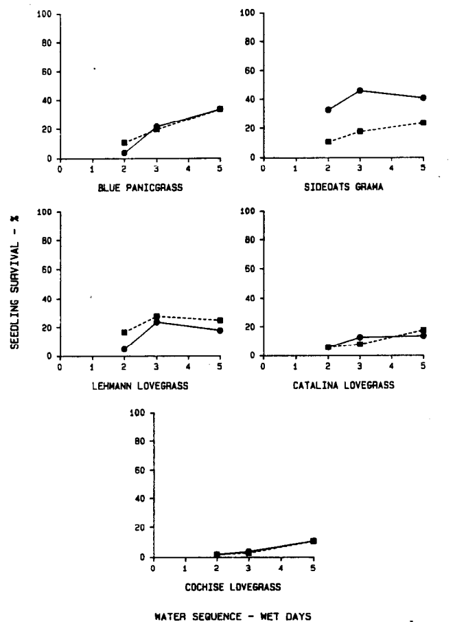
Fig. 7. Actual seedling survival in field plots and estimated seedling survival based on greenhouse results of 5 grass species for 2, 3, and 5 wet days followed by 5 dry days. Greenhouse data normalized by the corresponding field water sequence germination rates.
