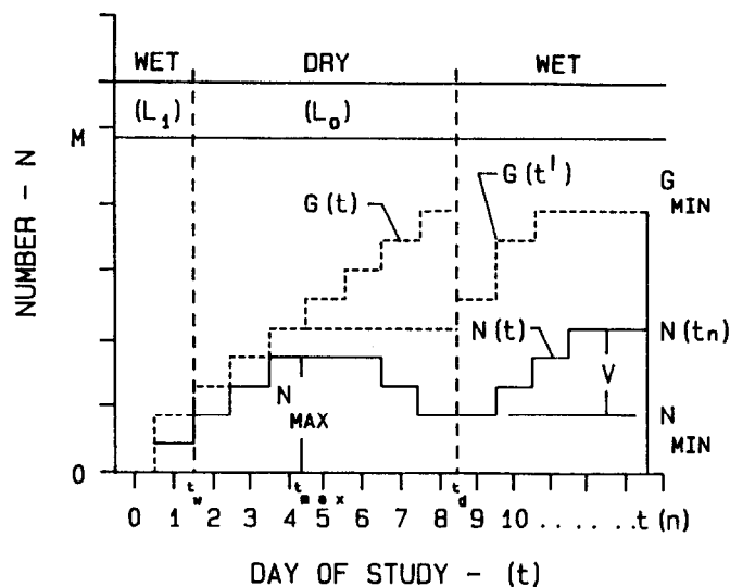
Fig. 1. Definition sketch of seed germination and seedling emergence response to the first wet-dry watering sequence following planting.
