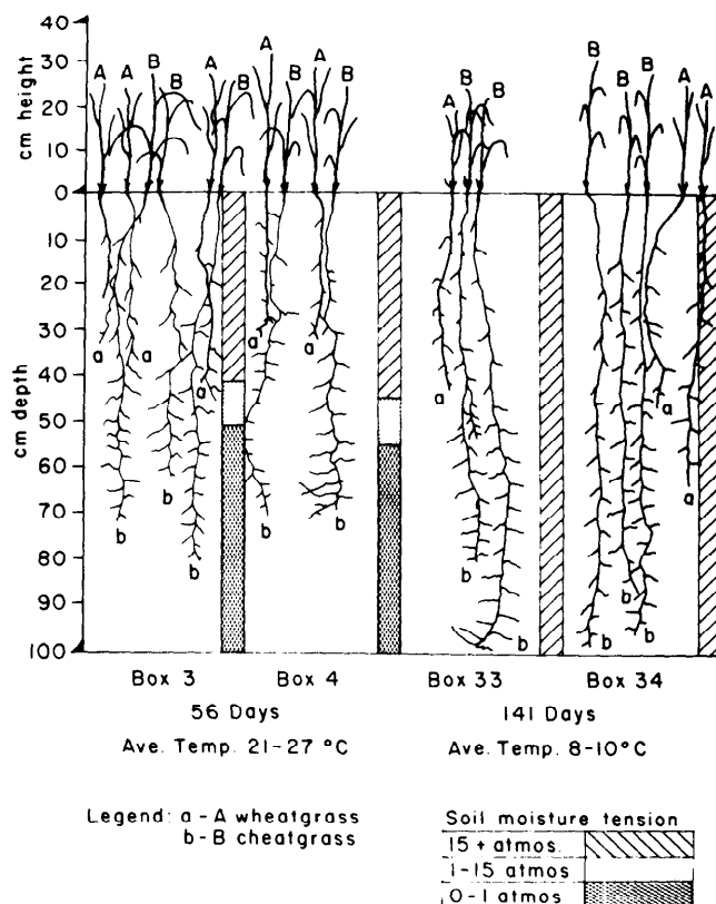
Fig. 2. Development of bluebunch wheatgrass and cheatgrass seedlings in relation to available soil water. Two replications of each run at room temperature and winter temperature in high density cheatgrass. (Used by permission of the Ecological Society of America; from Harris, 1967.)
