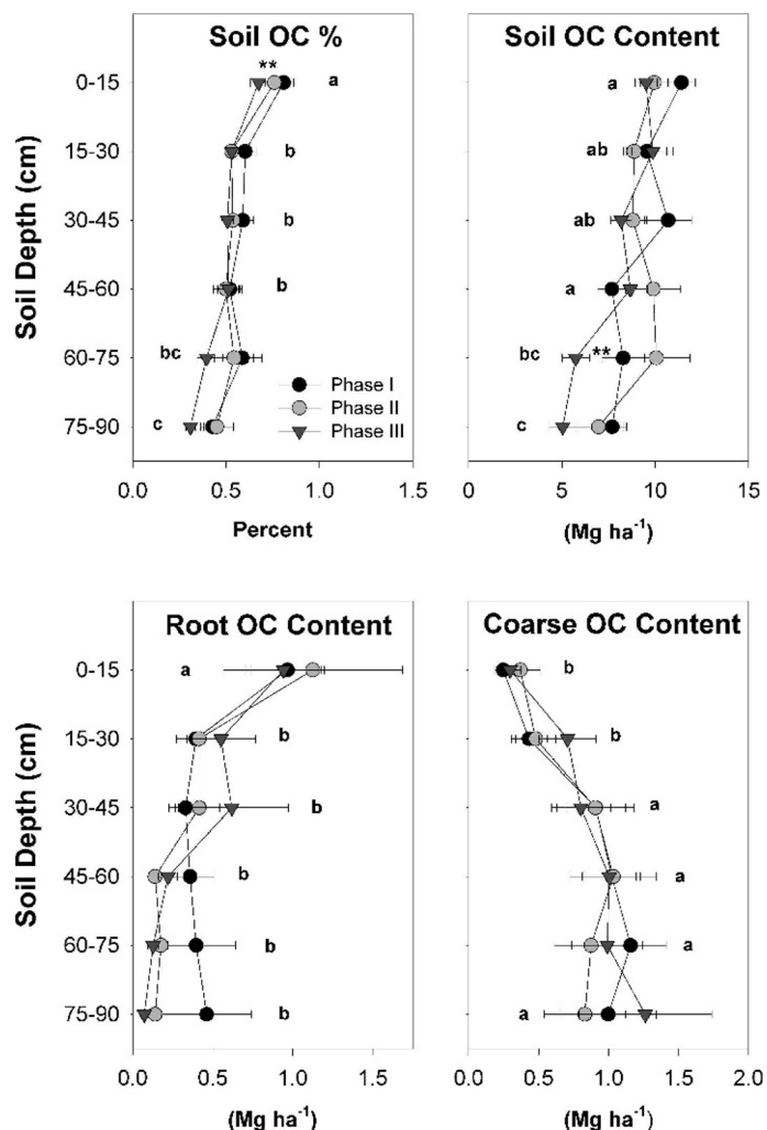
Figure 4. Means and standard errors by phase of cheatgrass invasion and soil depth increment for percent soil organic carbon, soil organic carbon content, root organic carbon content, and coarse fragment organic carbon content. Lowercase letters represent statistical groups for differences determined by the depth term in the generalized linear mixed model and Tukey's means comparisons ( P < 0.05 ). Means with different letters are statistically different. Asterisks indicate differences determined by the phase by depth interaction term in the generalized linear mixed model and Tukey's means comparisons ( P < 0.05 ).
