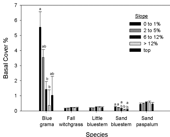
Figure 2. Basal cover of blue grama, fall witchgrass, little bluestem, sand bluestem, and sand paspalum as affected by slope gradient at the Southern Plains Experimental Range, Woodward, OK. Data averaged over stocking rate and year. Bars are standard errors. Different letters designate significant differences among slope categories ( P \leq 0.05 ).
