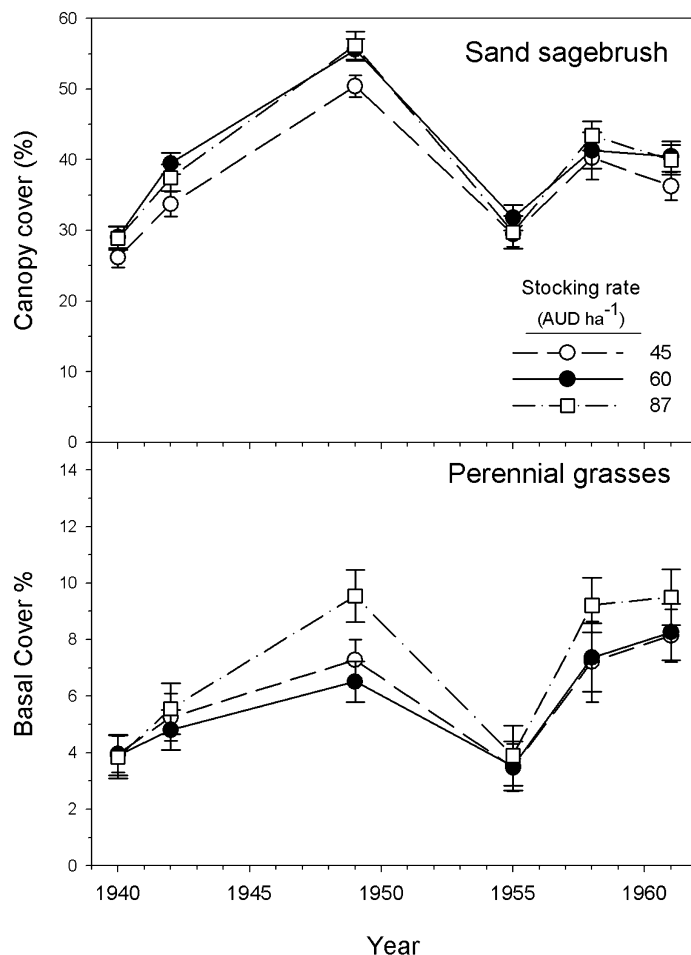
Figure 4. Canopy cover of sand sagebrush and basal cover of perennial grasses as affected by the interaction of stocking rate and year at the Southern Plains Experimental Range, Woodward, OK. Data are averaged over slope gradient. Bars are standard errors. Main effect of stocking rate is significant for sand sagebrush ( P = 0.05 ) but not perennial grasses ( P = 0.46 ). The stocking rate by year interaction is not significant for either component ( P = 0.80 for sand sagebrush; P = 0.29 for perennial grasses).
