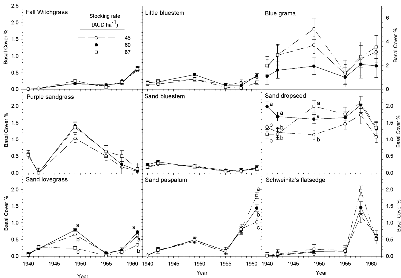
Figure 5. Basal cover of grasses as affected by the interaction of stocking rate and year at the Southern Plains Experimental Range, Woodward, OK. Data are averaged over slope gradient. Bars are standard errors. Different letters designate significant differences among stocking rates within year ( P \leq 0.05 ). Note different scale for cover of blue grama.
