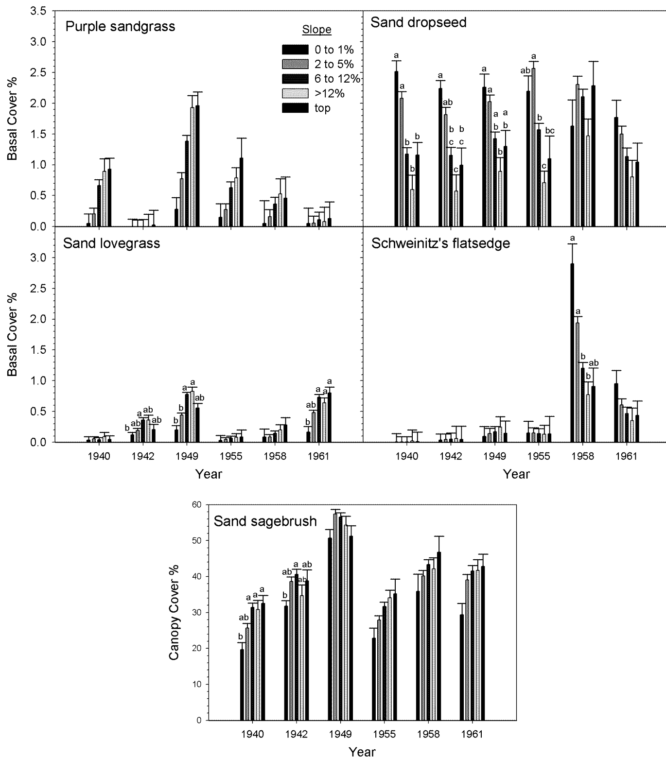
Figure 3. Basal cover of purple sandgrass, sand lovegrass, sand dropseed, and Schweinitz's flatsedge, and canopy cover of sand sagebrush as affected by the interaction of slope gradient and year at the Southern Plains Experimental Range, Woodward, OK. Data averaged over stocking rate. Bars are standard errors. Different letters designate significant differences among slope categories within year ( P \leq 0.05 ).
