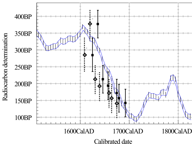
Figure 10 Measured ^{14}\text{C} data of the Arhat #8 statue (solid bars) and those corrected by dendro-dates (dotted bars) are compared with IntCal04 calibration curve.
