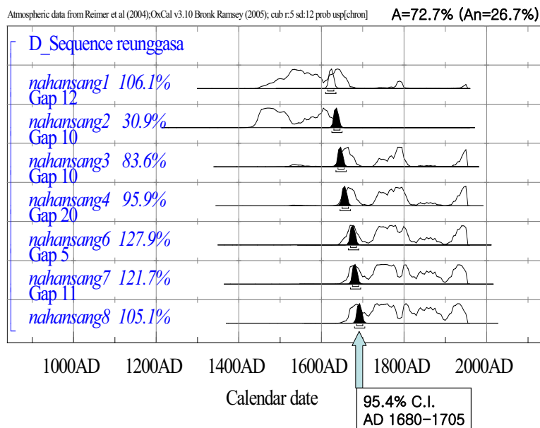
Figure 9 Probability distribution profiles (in black) of ^{14}\text{C} dates for each of the 7 individual samples from the Arhat nahansang statue after wiggle-matching.
