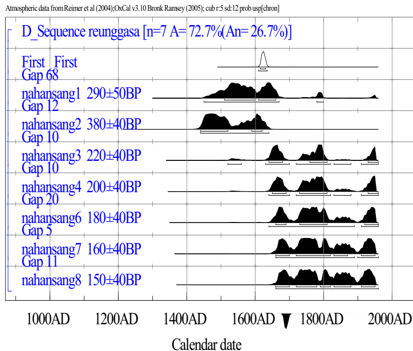
Figure 8 Probability distribution profiles of ^{14}\text{C} dates for each of 7 individual samples from the Arhat nahansang statue prior to wiggle-matching (the probability distribution of each sample is given in black profile, under which the 68.2% and 95.4% confidence intervals are designated with bars).
